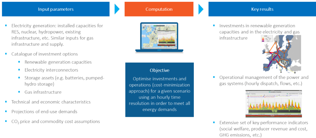
Figure 11 – Modelling approach in Artelys Crystal Super Grid
